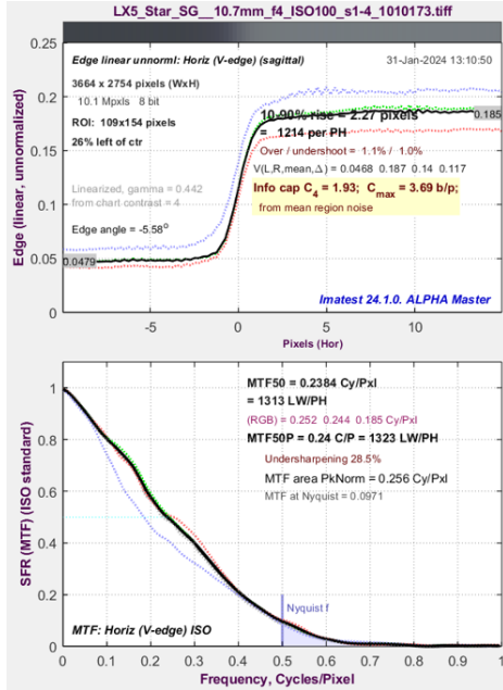
Figure 8. Edge and SFR (MTF) plot for compact digital camera for an unsharpened TIFF from raw. Upper: Mean edge \mu_s(x) . Lower: SFR(f) . C_4 is the Shannon information capacity for a 4:1 contrast ratio edge.
